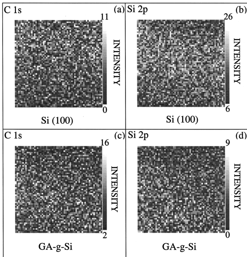
Figure 5. C 1s and Si 2p chemical maps in a 0.3 \text{ mm} \times 0.3 \text{ mm} area of the pristine Si(100) surface (a, b) and the GA- g -Si surface ([epoxide]/[Si] = 0.3) (c, d).
