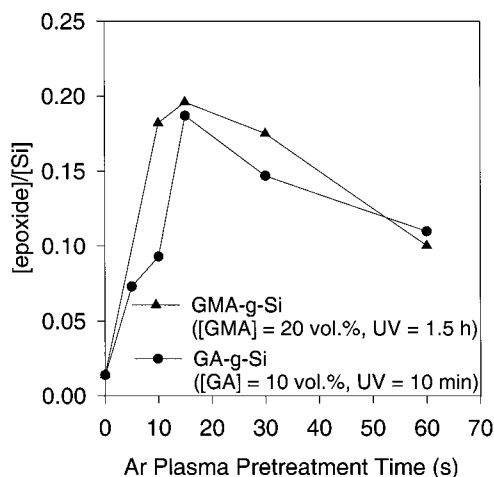
Figure 3. Effect of the Ar plasma pretreatment time of the Si(100) substrate on the graft concentration, expressed as the [epoxide]/[Si] ratio of the GA and GMA polymer.
