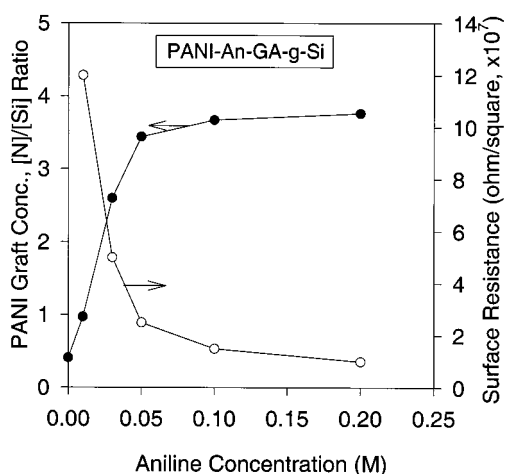
Figure 8. Effect of aniline monomer concentration used during the oxidative graft polymerization on the graft concentration of PANI, expressed as the [N]/[Si] ratio, on the PANI-An-GA- g -Si surface and on the corresponding surface resistance.
