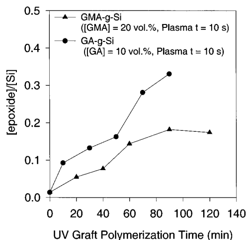
Figure 4. Effect of UV-induced graft copolymerization time on the graft concentration, expressed as the [epoxide]/[Si] ratio of the GA and GMA polymer.
