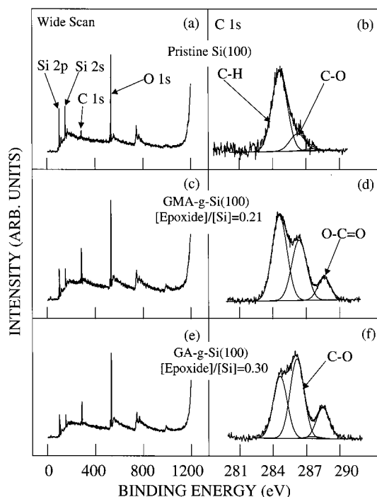
Figure 2. Wide scan and C 1s core-level spectra of the pristine Si(100) surface (a, b), 10 s Ar plasma-pretreated Si(100) surface after the UV-induced graft copolymerization in 20 vol % GMA solution for 1.5 h (c, d), and 15 s Ar plasma-pretreated Si(100) surface after the UV-induced graft copolymerization in 20 vol % GA solution for 15 min (e, f).
