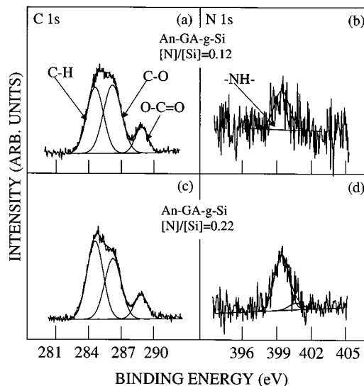
Figure 6. C 1s and N 1s core-level spectra of the GA- g -Si surface ([epoxide]/[Si] = 0.3) after reaction with aniline at 30^\circ\text{C} for 4 h in pure An (a, b) and in 60 vol % ethanol solution of aniline (c, d).
